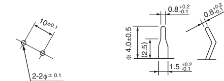
(PC board hole dimensions)
