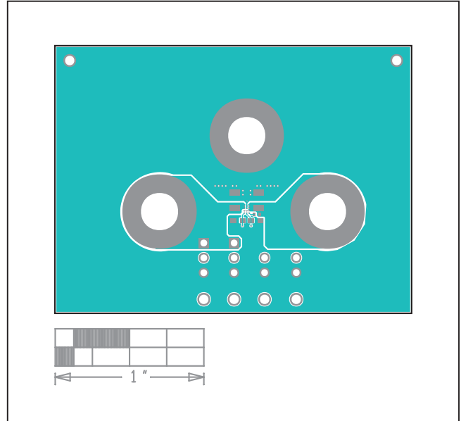
MAX38913A WLP EV Kit PCB Layout—Top
