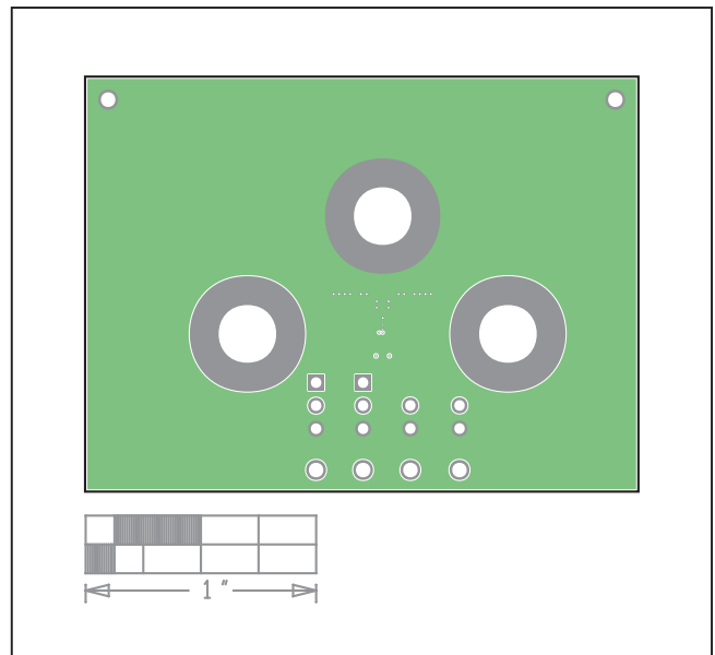
MAX38913A WLP EV Kit PCB Layout—Layer 3
