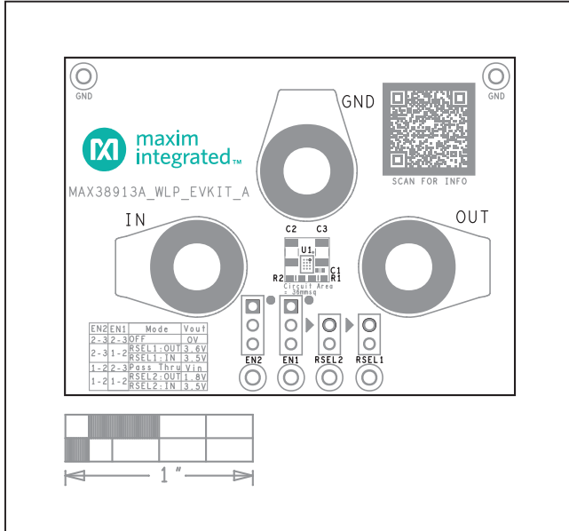
MAX38913A WLP EV Kit Component Placement Guide—Top Silkscreen
