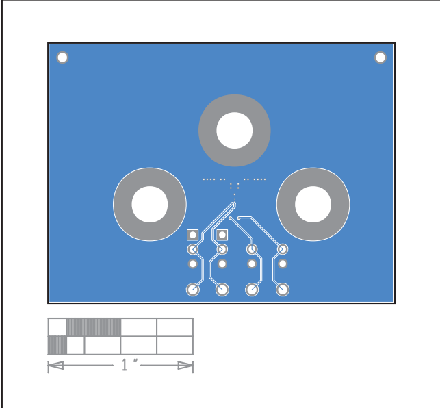
MAX38913A WLP EV Kit PCB Layout—Bottom
