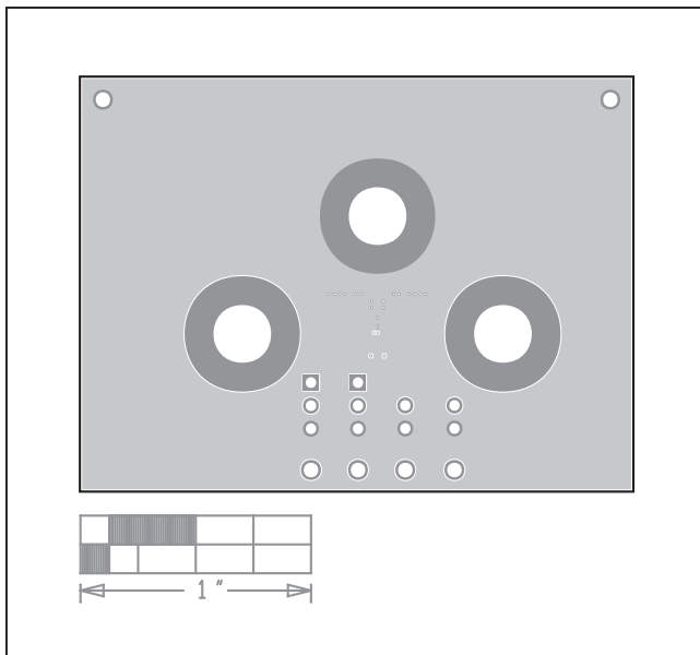
MAX38913A WLP EV Kit PCB Layout—Layer 2
