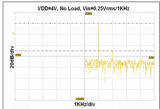
Figure 21: Audio-Band Output Spectrum
