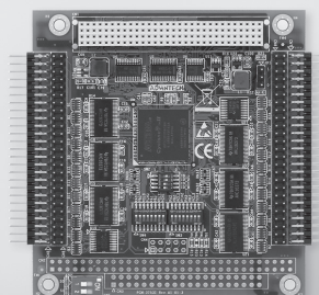
PCM-3753I
