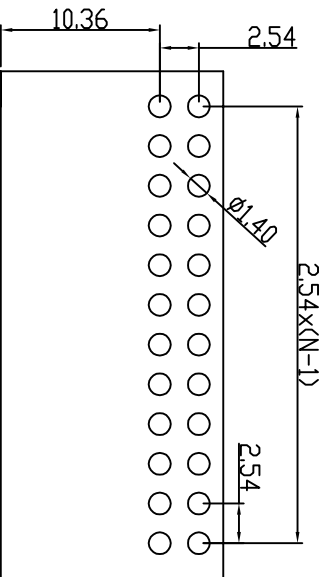
PCB LAYOUT
