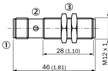
All dimensions in mm (inch)
