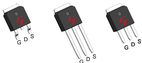
TO-252-2L
