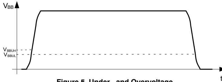
Figure 5. Under- and Overvoltage
