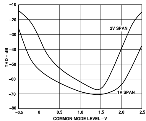
d. Single-Ended Input, 5 V Supplies
