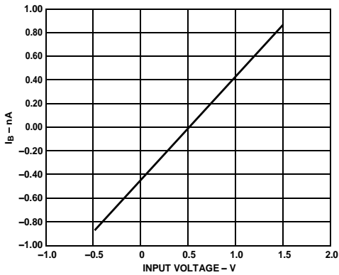
Figure 5. Input Bias Current vs. Input Voltage
