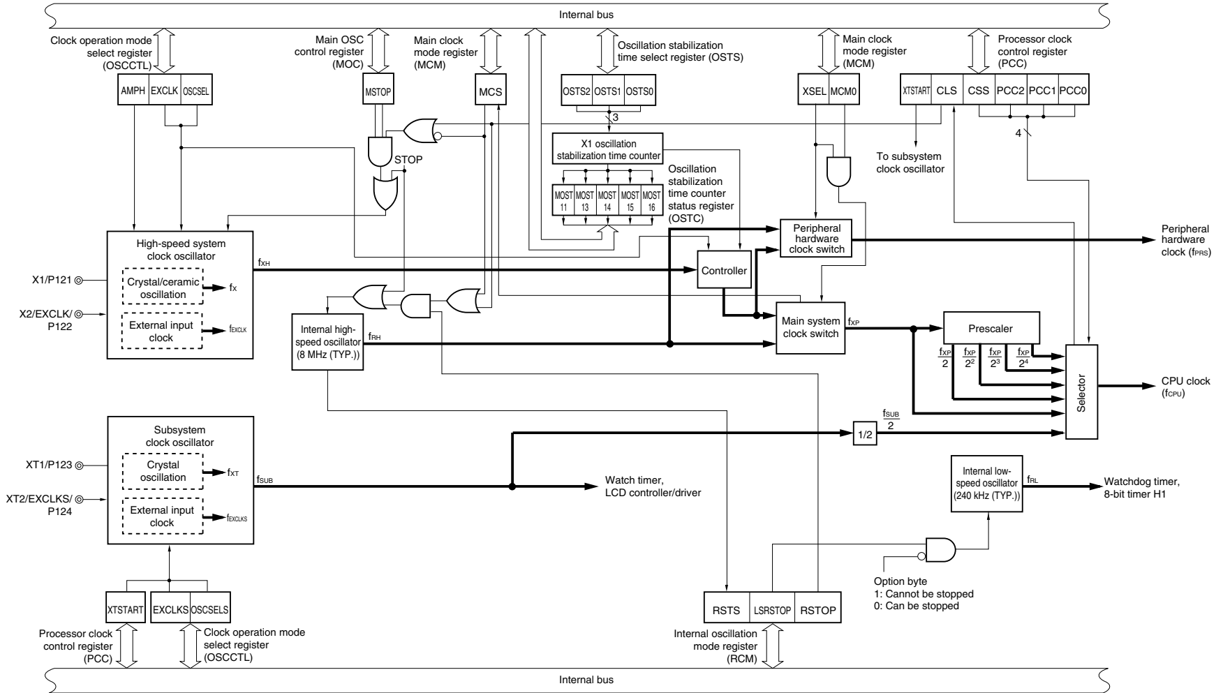
<R> Figure 6-1. Block Diagram of Clock Generator
