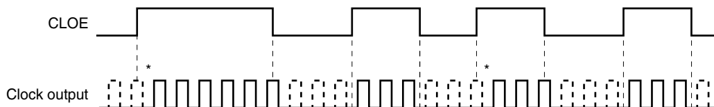
Figure 12-4. Clock Output Application Example
