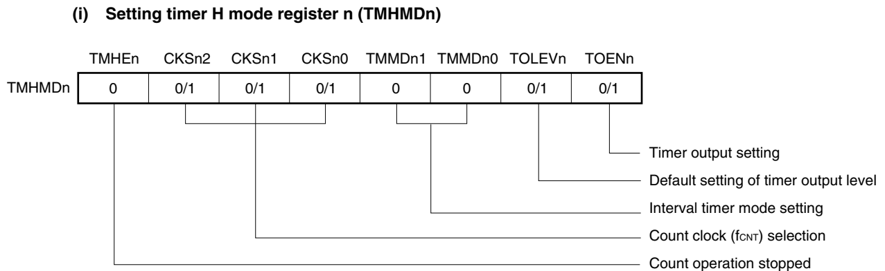
Figure 9-9. Register Setting During Interval Timer/Square-Wave Output Operation
