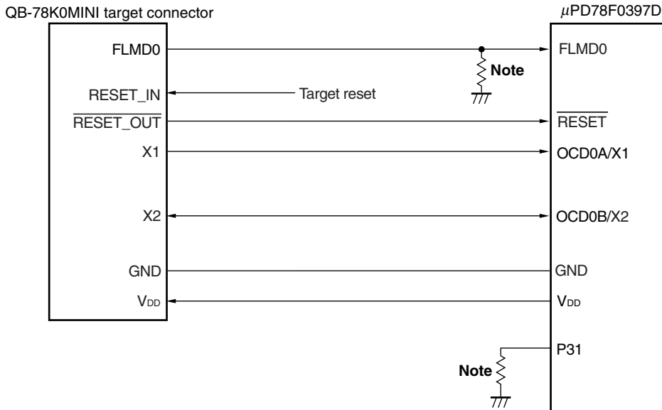
Figure 28-1. Connection Example of QB-78K0MINI and μPD78F0397D (When OCD0A/X1 and OCD0B/X2 Are Used)
