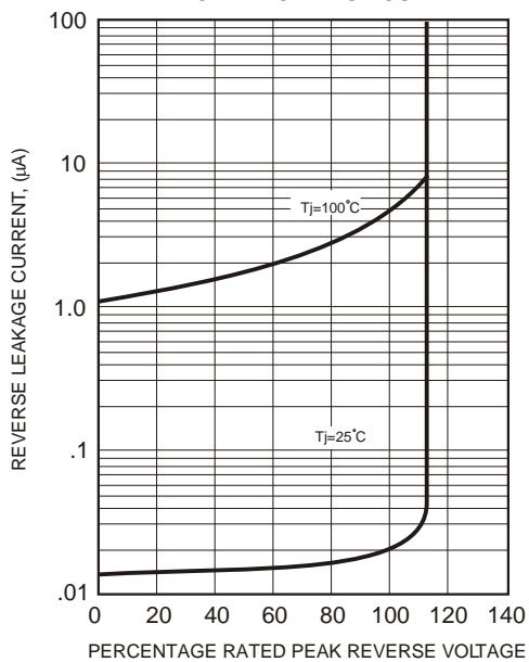
CHARACTERISTICS
