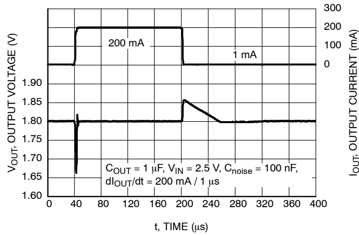
Figure 27. Load Transient Response, V_{OUT} = 1.8 V , C_{OUT} = 1 \mu F , C_{noise} = 100 nF
