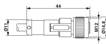
M12 x 1 socket, straight
