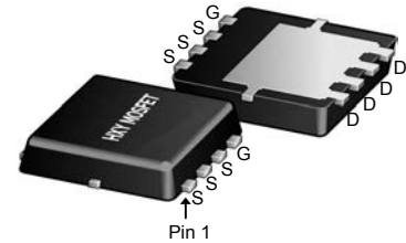
DFN5X6-8L (DFN-8(5.1x5.8))
