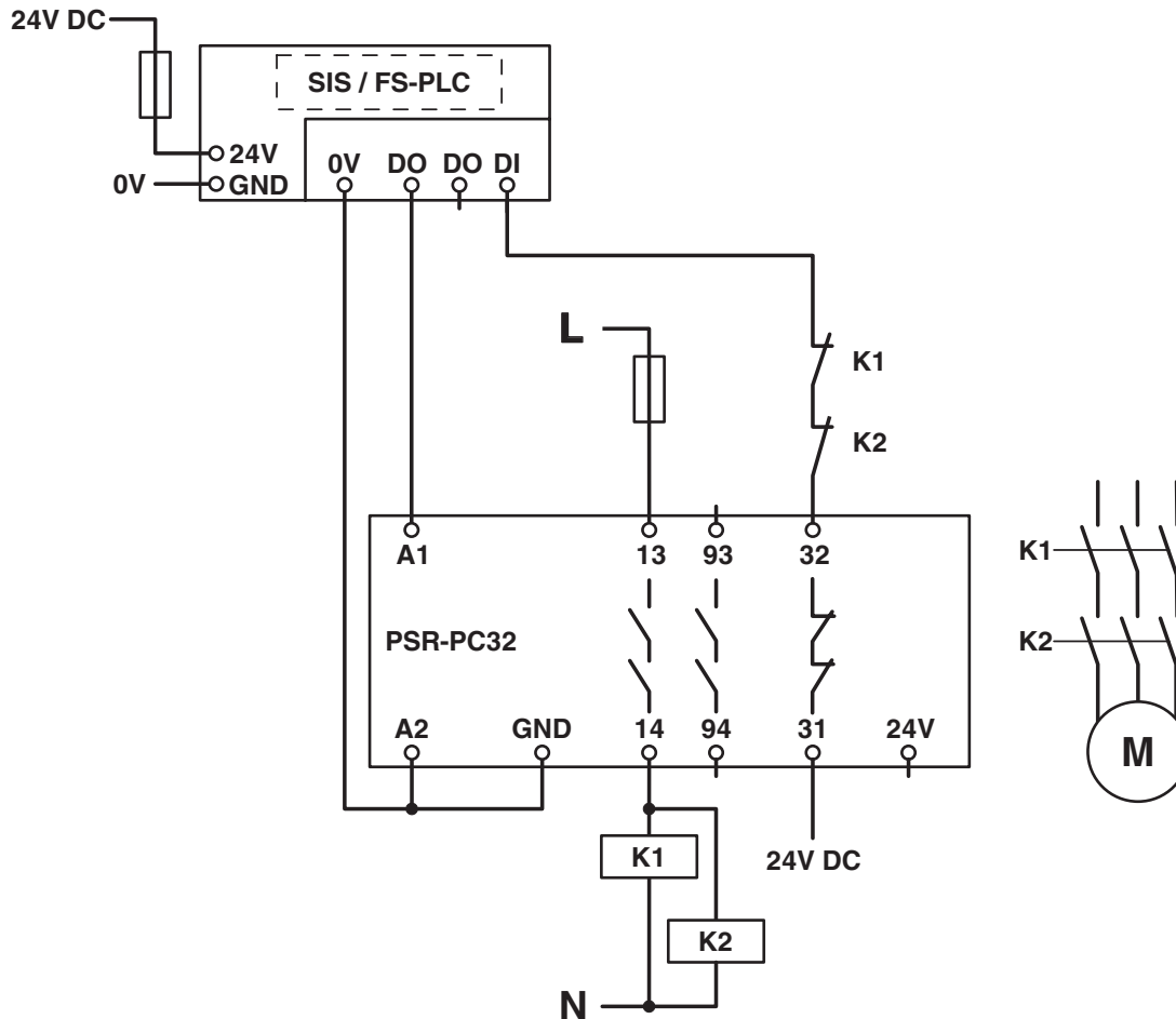
Circuit diagram
