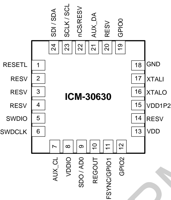
Figure 3. Pin out Diagram for ICM-30630 3x3x1mm LGA
