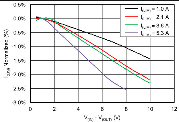
Figure 20. Current Limit Normalized (%) vs V_{(IN)} - V_{(OUT)} Thermal shutdown occurs when I_{(LIM)} = [V_{(IN)} - V_{(OUT)}] > 8\text{ V} 5.3 A
