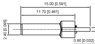
SECT B-B
