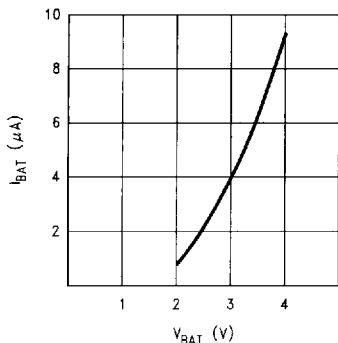
FIGURE 9-21. Typical Battery Current during Battery Backed Mode
