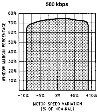
FIGURE 5-2. PC87323 Dynamic Window Margin Performance
