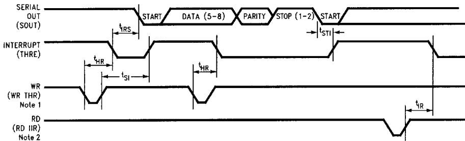
FIGURE 11-6. Transmitter Timing
