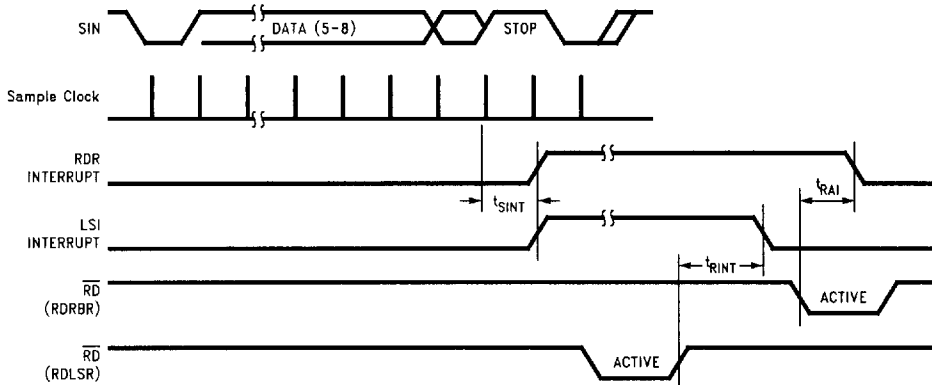
FIGURE 11-8. Receiver Timing
