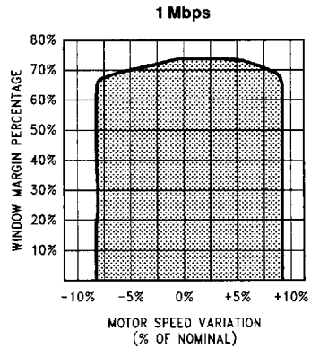
FIGURE 5-2. PC87323 Dynamic Window Margin Performance
