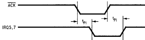
FIGURE 11-18. Compatible Mode Parallel Port Interrupt Timing
