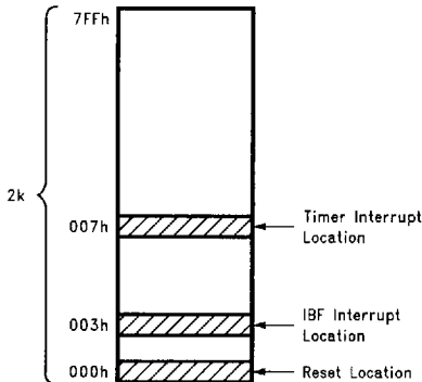
FIGURE 9-4. Keyboard Controller Program Memory Map
