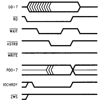
FIGURE 7-5. EPP 1.9 Address Read
