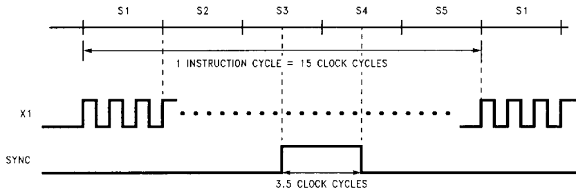
FIGURE 9-13. Instruction Cycle Timing
