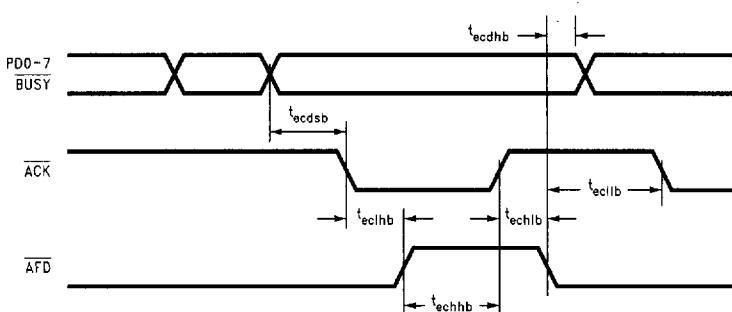
FIGURE 11-23. ECP Parallel Port Backward Timing Diagram
