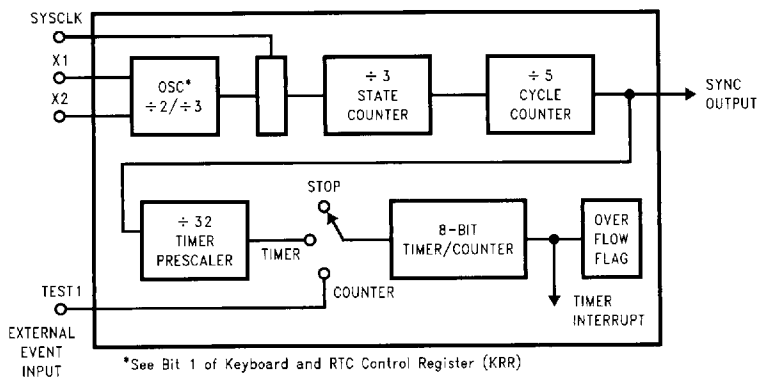
FIGURE 9-10. Timing Generation and Timer Circuit
