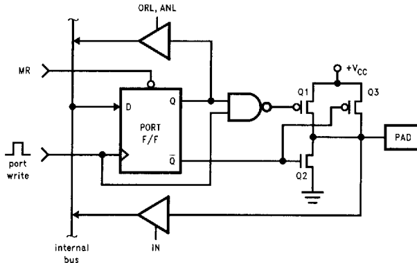
FIGURE 9-8. Active Pull-Up I/O Port Structure
