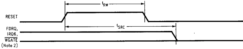
FIGURE 11-13. Reset Timing
