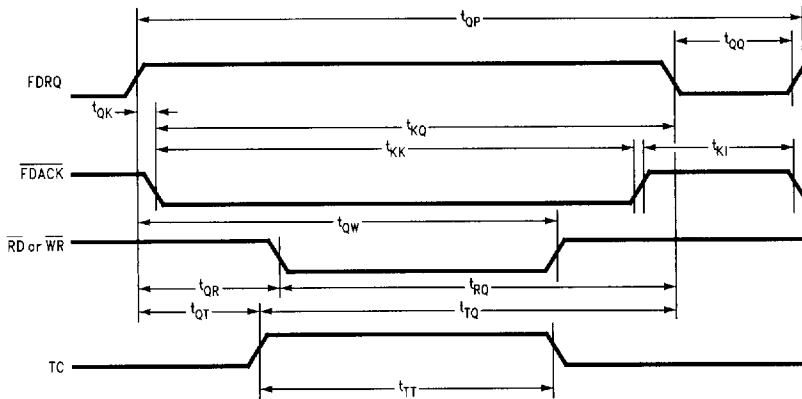
FIGURE 11-12a. FDC DMA Timing
