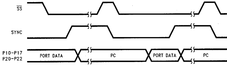
FIGURE 9-15. Single-Step Operation
