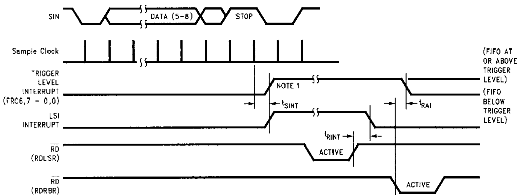
FIGURE 11-8. Receiver Timing
