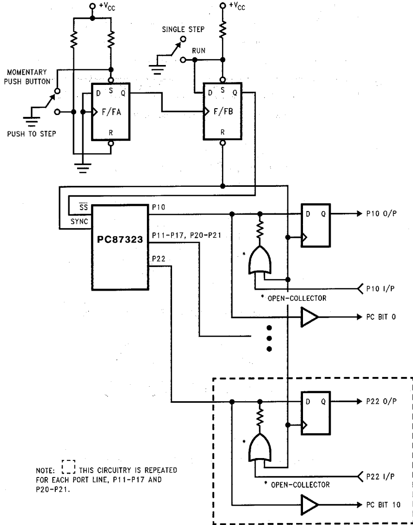
FIGURE 9-14. Example of Single-Step Circuit
