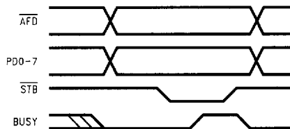
FIGURE 7-6. ECP Forward Write Cycle
