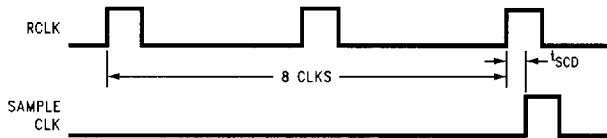
FIGURE 11-7. Sample Clock Timing
