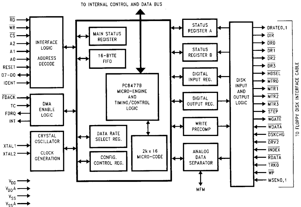
FIGURE 3-1. FDC Functional Block Diagram
