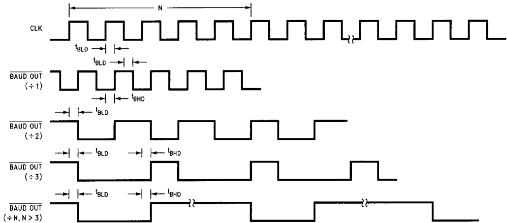
FIGURE 11-5. Baud Out Timing
