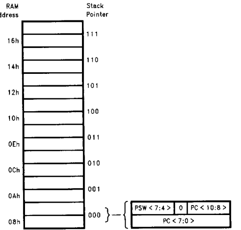
FIGURE 9-6. Keyboard Controller Stack Organization
