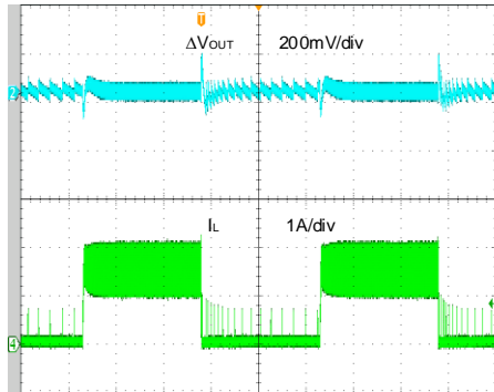
Load Transient ( V_{IN} = 12V, V_{OUT} = 3.3V, I_{OUT} = 0A \sim 1.5A )
