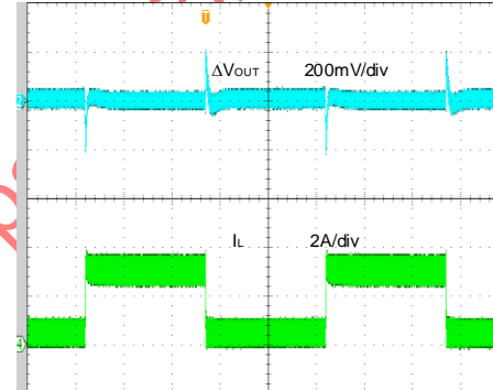
Load Transient ( V_{IN} = 12V, V_{OUT} = 3.3V, I_{OUT} = 0.3A \sim 3A )
