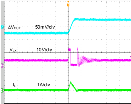
Output Ripple ( V_{IN} = 12V, V_{OUT} = 3.3V, I_{OUT} = 0A )
