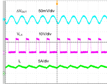
Output Ripple ( V_{IN} = 12V, V_{OUT} = 3.3V, I_{OUT} = 3A )
