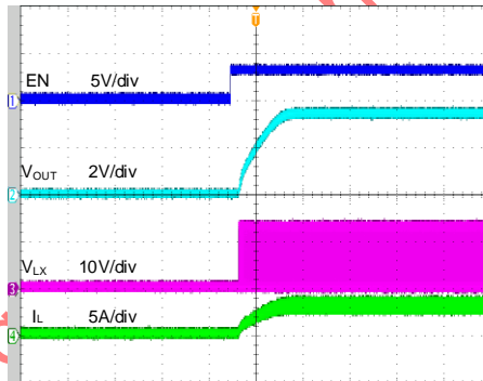
Startup from Enable ( V_{IN} = 12V, V_{OUT} = 3.3V, I_{OUT} = 3A )
