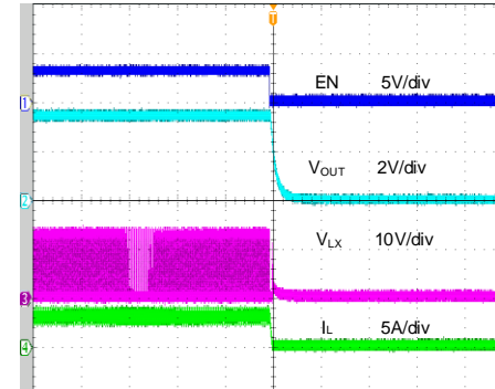
Shutdown from Enable ( V_{IN} = 12V, V_{OUT} = 3.3V, I_{OUT} = 3A )
