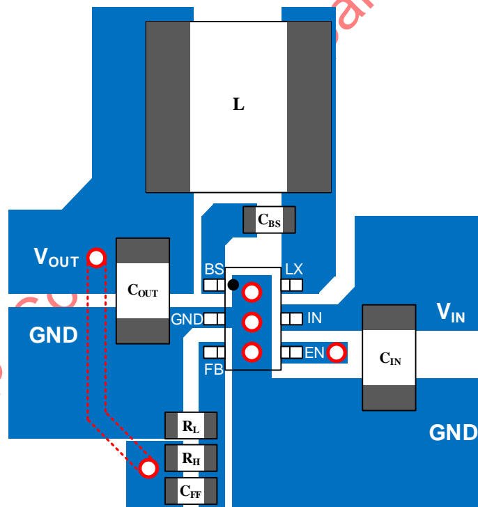
Figure9. Suggested PCB Layout
