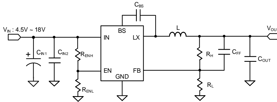
Figure8. Schematic Diagram
