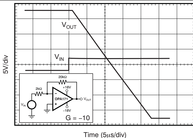
Figure 26. Positive Overload Recovery
