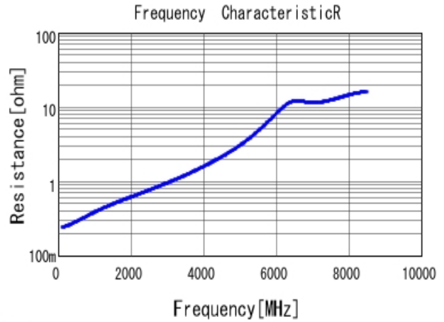
GCM1885C1H100JA16 R DCOV, 25degC
