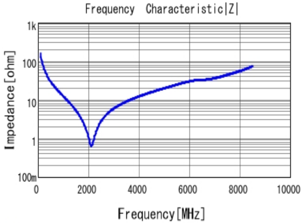
GCM1885C1H100JA16 |Z| DCOV, 25degC
