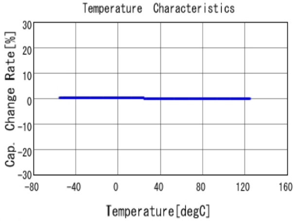
■ GCM1885C1H100JA16 C-Temp. capchange, DCOV, AC1Vrms
