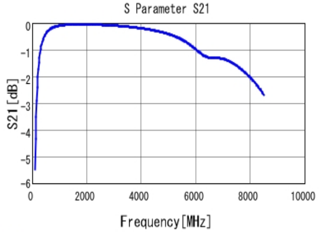
■ GCM1885C1H100JA16 S21 DCOV, 25degC
