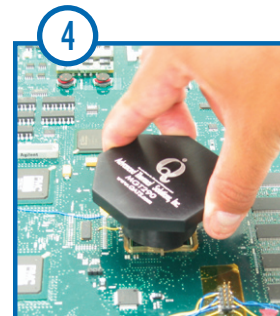
Position the Knob Tool with Frame Clip over the component, rotate 45° counter-clockwise releasing the Frame Clip
