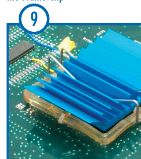
Inspect the installation. Double check to make sure the Heat Sink is securely attached.
