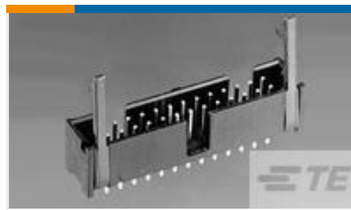
TE Part #2-1761609-3 IDC LOW PRO HDR 10P RA SHT LAT
