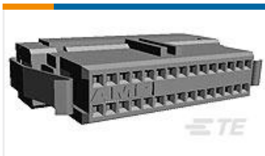
TE Part #2-111196-1 50 RCPT SYSTEM 50, LEAD FREE
