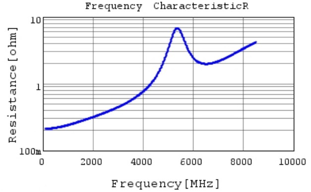
GCM1555C1H100FA16 R DCOV,25degC
