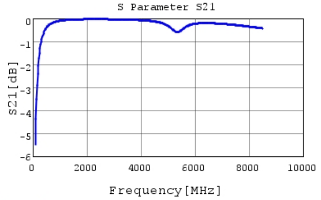
GCM1555C1H100FA16 S21 DCOV, 25degC
