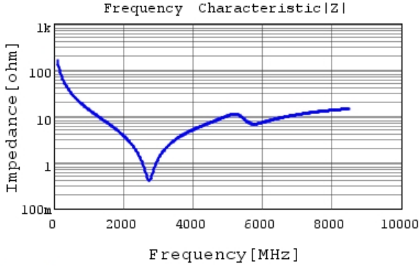
GCM1555C1H100FA16 |Z| DCOV,25degC
