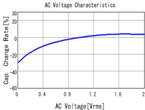
■ GRM033R61C104KE18 C-AC Voltage capchange, DCOV, 25.0d
