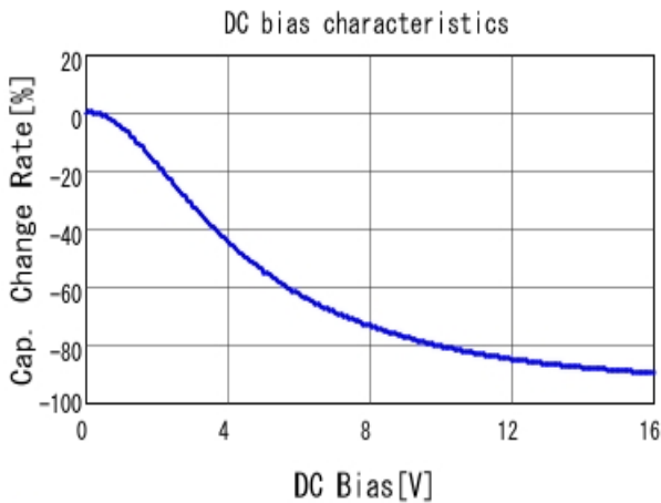
■ GRM033R61C104KE18 C-DC bias capchange, 25.0degC, AC1V
