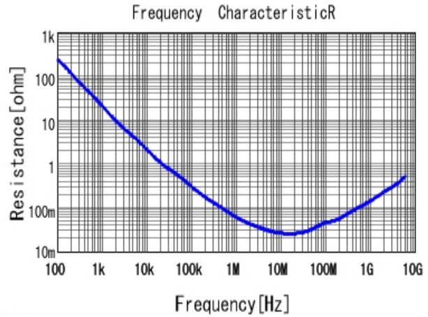
■ GRM033R61C104KE18 R DCOV, 25degC
