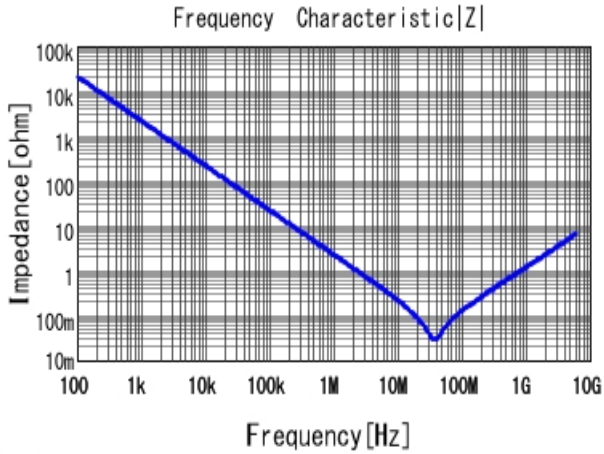
■ GRM033R61C104KE18 |Z| DCOV, 25degC
