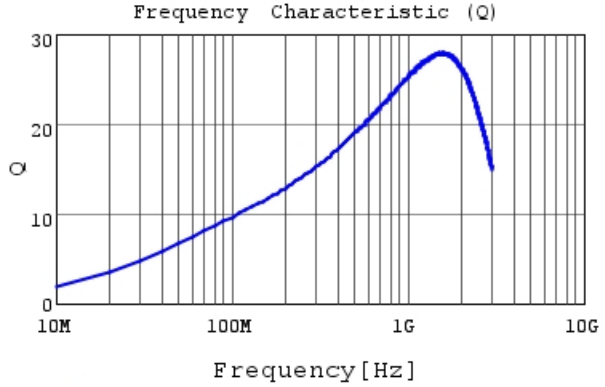
LQP03TN12NH02 Q
