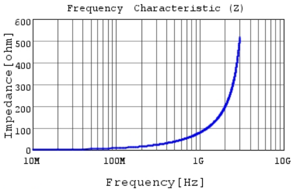
LQP03TN12NH02 |Z|
