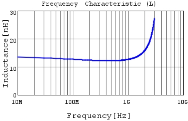
LQP03TN12NH02 L
