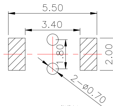
PCB.WELDING DRAWING
