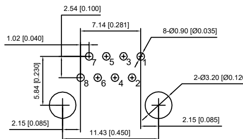
RECOMMENDED PCB LAYOUT VIEWED FROM COMPONENT SIDE
