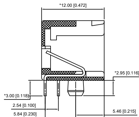
CUTAWAY VIEW
