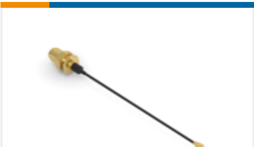
TE Part #2016693-4 RF CA,UMCC1 TO RPSMA JACK,1.13 MM,L200MM
