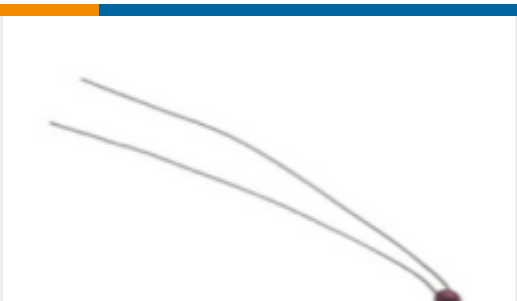
TE Part #GA100K6A1B DISCRETE 100K OHMS, +/-0.2C 0C TO 70C
