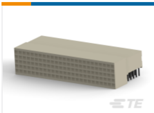
TE Part #5352171-1 HM Receptacle Connector: Traditional Backplane, Coplanar, 2mm
