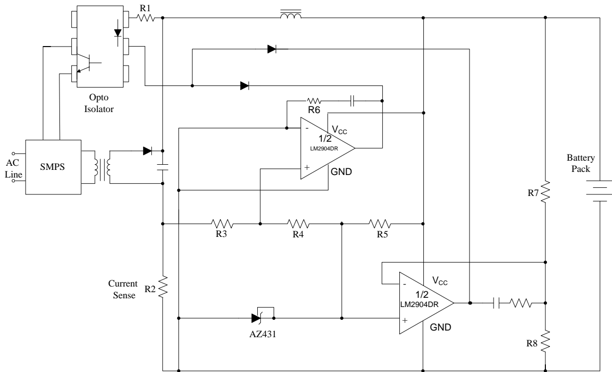
Battery Charger
