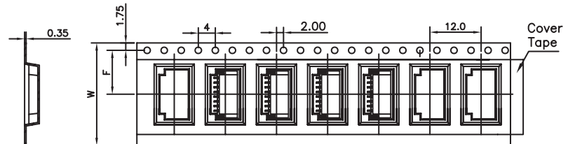
For Reel width (dimension W) 16,24mm Single row hole
