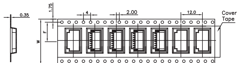
For Reel width (dimension W) 32,44,56,72mm Double rows hole
