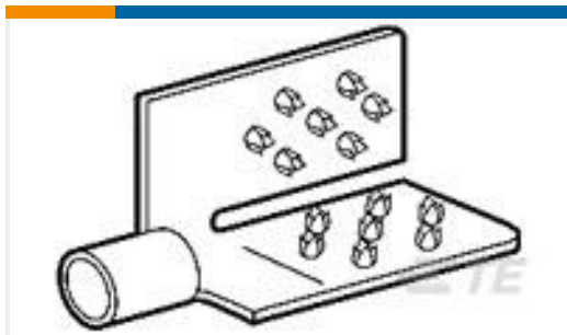
TE Part #1-330716-2 TERMINAL,TERMI-FOIL 12-10
