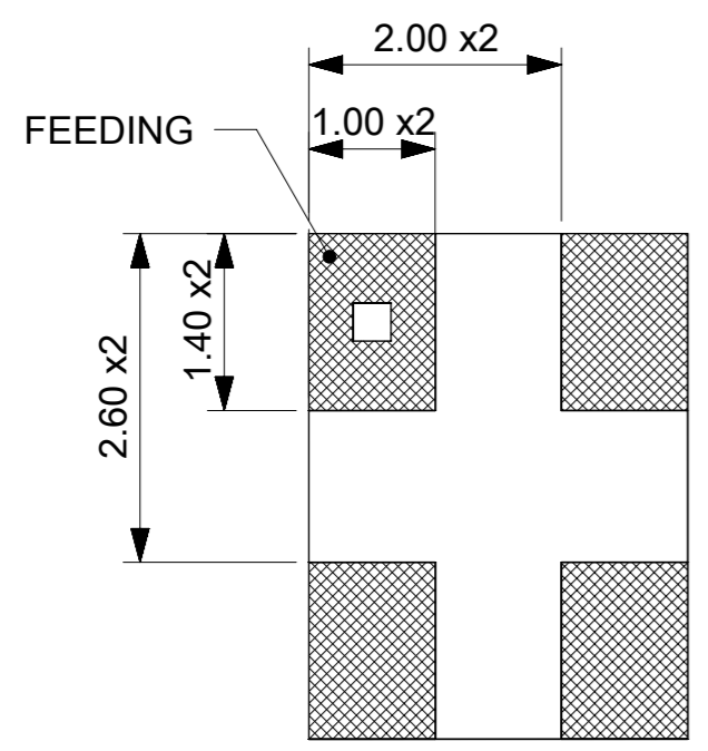
PADS OF PRODUCT FOR SOLDER BOTTOM VIEW
