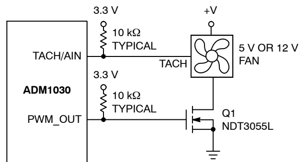
Figure 34. Interfacing the ADM1030 to a 3-wire Fan
