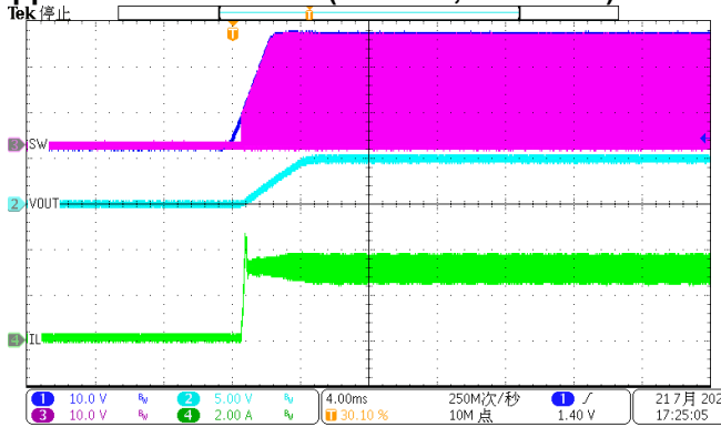
Figure 12. Power Up, IOU=3A
