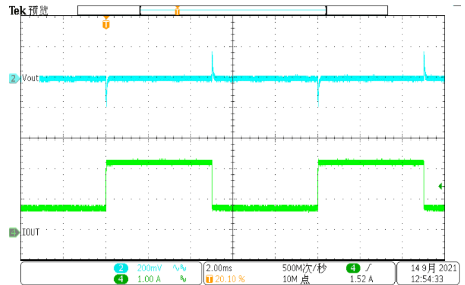
Figure 17. Load Transient IOU=0.75A to 2.25 A, SR=1600mA/us
