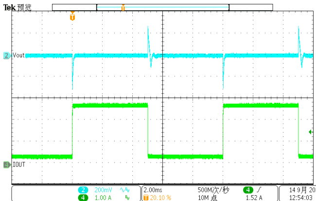
Figure 16. Load Transient IOU=0.3A to 2.7A, SR=1600mA/us
