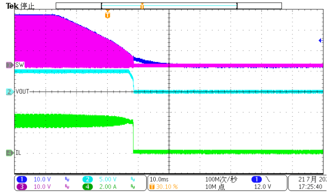
Figure 13. Power Down, IOU=3A
