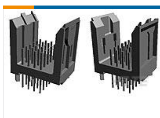
TE Part #5536501-3 2MM FB,ASY,96,SIG,HDR,SL,4.25
