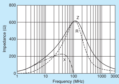
BLM31PG601SZ1/BLM31PG601SH1
