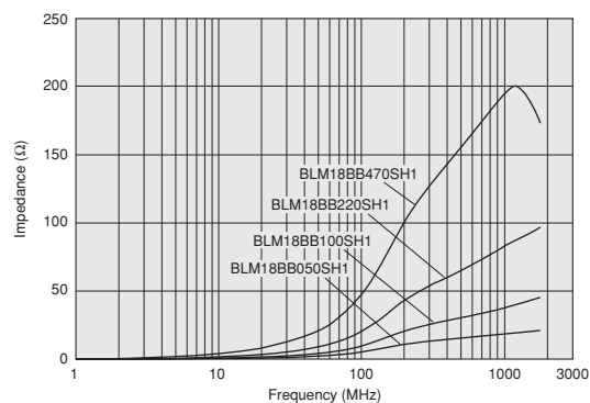
BLM18BB_SH Series (5Ω~47Ω)
