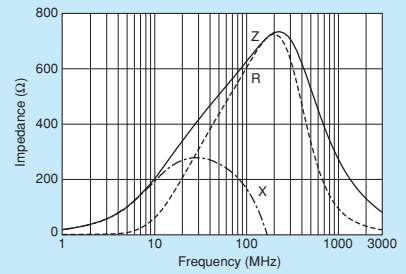
BLM15AG601SZ1/BLM15AG601SH1
