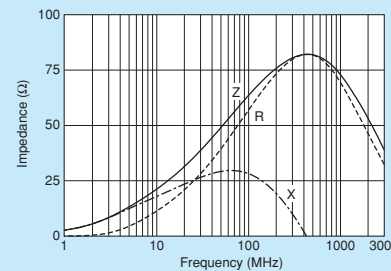
BLM18PG600SZ1/BLM18PG600SH1
