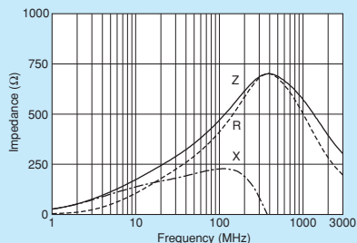
BLM18HG471SZ1/BLM18HG471SH1
