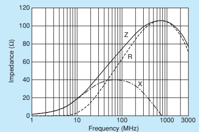
BLM15AX700SZ1
