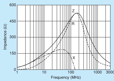
BLM21AG471SZ1/BLM21AG471SH1
