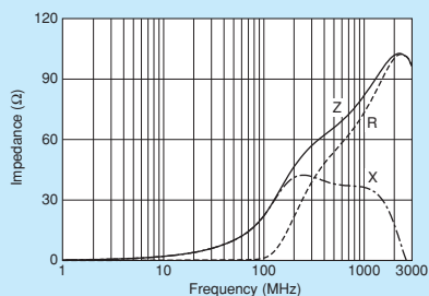
BLM18BB220SZ1/BLM18BB220SH1
