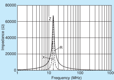
NFZ32BW621HZ10
