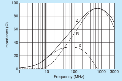
BLM15PD600SZ1
