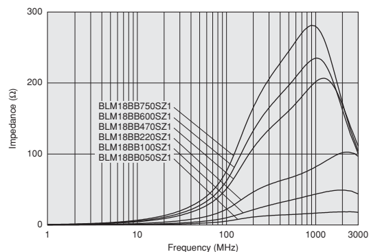
BLM18BB_SZ Series (5Ω~75Ω)
