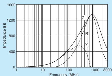
BLM18HD471SZ1/BLM18HD471SH1
