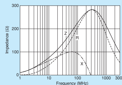
BLM18PG221SZ1/BLM18PG221SH1
