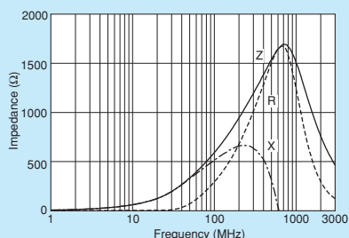
BLM18HD601SZ1/BLM18HD601SH1
