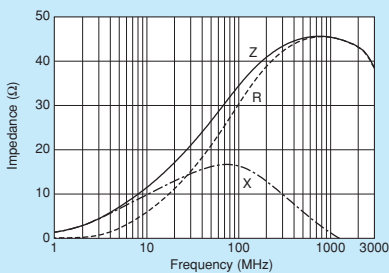
BLM31PG330SZ1/BLM31PG330SH1
