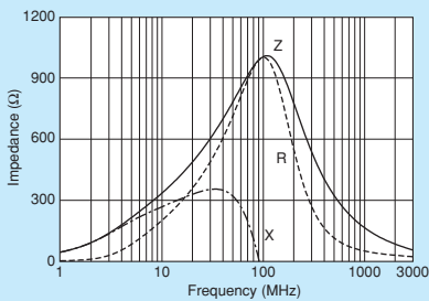
BLM21AG102SZ1/BLM21AG102SH1
