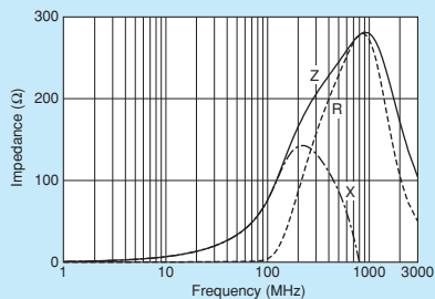
BLM18BB750SZ1/BLM18BB750SH1
