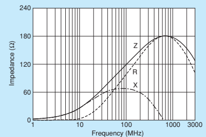
BLM03AX121SZ1
