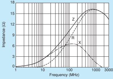
BLM15PG100SZ1
