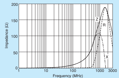
BLM18BA100SZ1/BLM18BA100SH1
