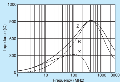
BLM18HG601SZ1/BLM18HG601SH1
