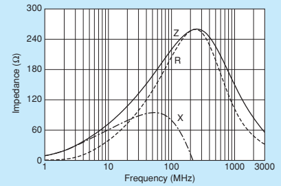
BLM21AG221SZ1/BLM21AG221SH1
