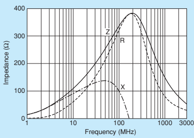
BLM21AG331SZ1/BLM21AG331SH1
