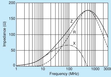
BLM15AG121SZ1
