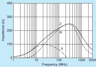
BLM18SG221TZ1
