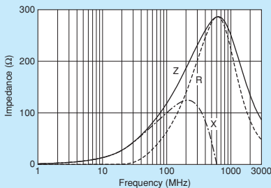
BLM18BD121SZ1/BLM18BD121SH1
