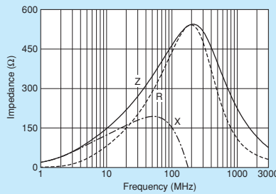
BLM18AG471SZ1/BLM18AG471SH1
