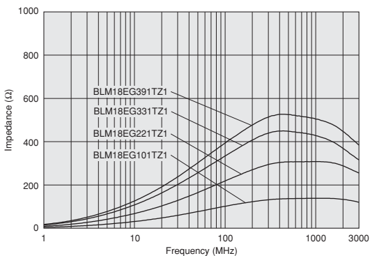
BLM18EG_TZ1 Series
