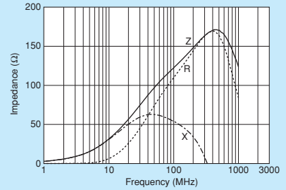
BLM15AG121SH1
