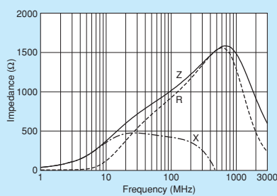
BLM15HG102SZ1/BLM15HG102SH1
