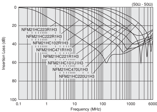
NFM21HC_1H3 Series
