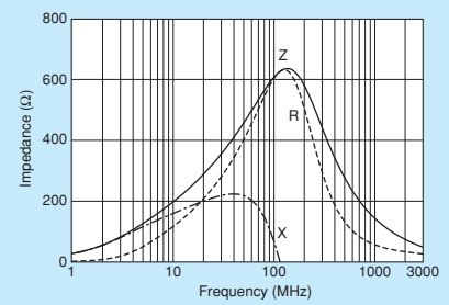
BLM21AG601SZ1/BLM21AG601SH1
