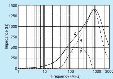
BLM15HD601SZ1/BLM15HD601SH1
