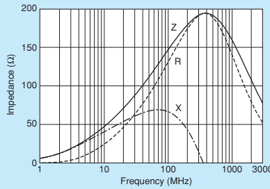
BLM18AG151SZ1/BLM18AG151SH1
