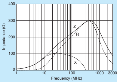
BLM15AG221SZ1
