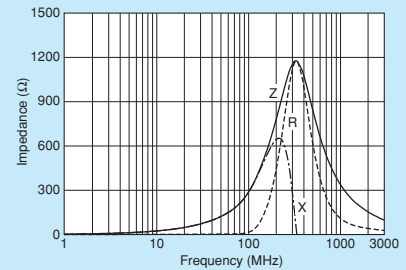
BLM18BB331SZ1/BLM18BB331SH1
