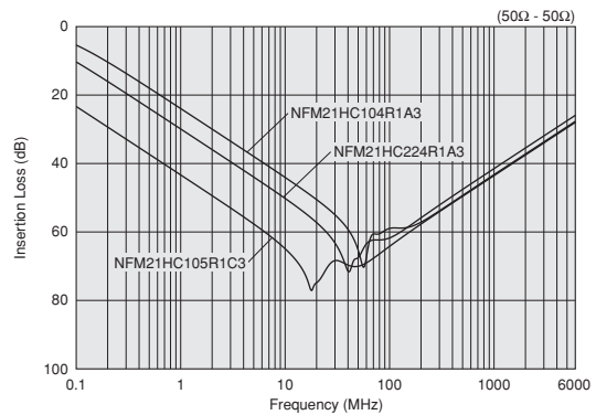
NFM21HC_1A3/1C3 Series
