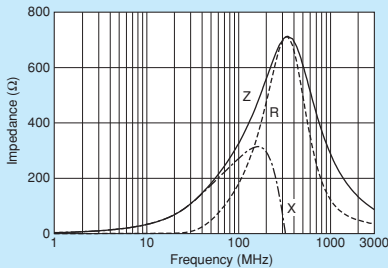
BLM18BD331SZ1/BLM18BD331SH1
