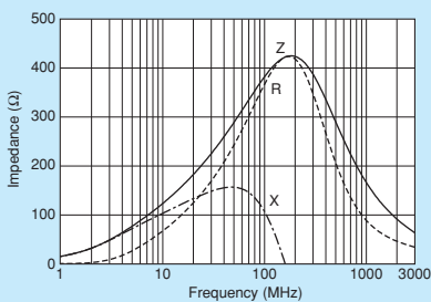
BLM31PG391SZ1/BLM31PG391SH1
