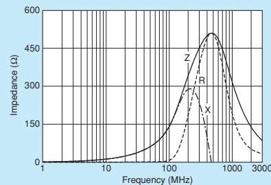
BLM18BB141SZ1/BLM18BB141SH1
