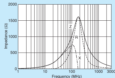
BLM18BD222SZ1/BLM18BD222SH1
