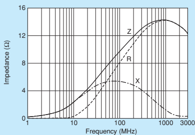
BLM03AX100SZ1
