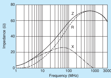
BLM31PG500SZ1/BLM31PG500SH1
