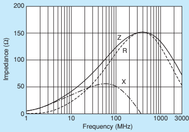
BLM21AG121SZ1/BLM21AG121SH1
