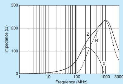
BLM18BB600SZ1/BLM18BB600SH1
