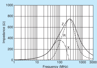
BLM15BD471SZ1/BLM15BD471SH1
