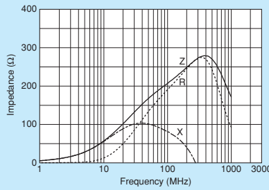
BLM15AG221SH1
