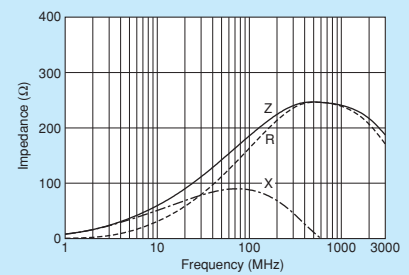
BLM18EG181SH1
