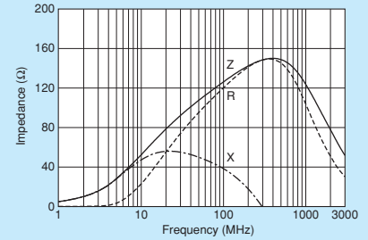
BLM18SG121TZ1
