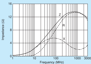
BLM15AX100SZ1
