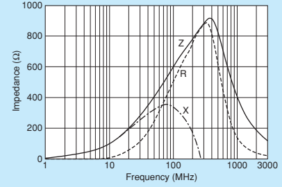
BLM03AG601SZ1
