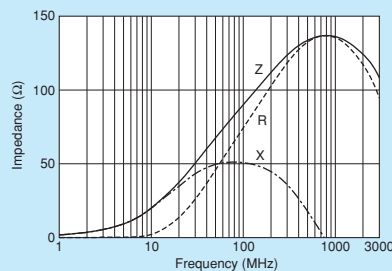
BLM03AX800SZ1
