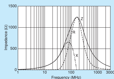
BLM15BD102SZ1/BLM15BD102SH1
