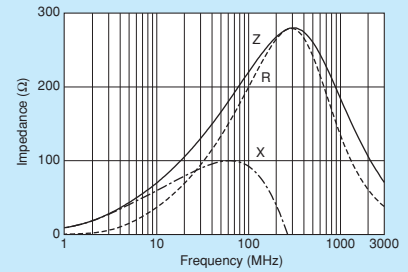
BLM18AG221SZ1/BLM18AG221SH1
