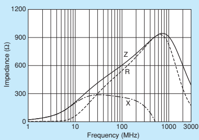
BLM15HG601SZ1/BLM15HG601SH1
