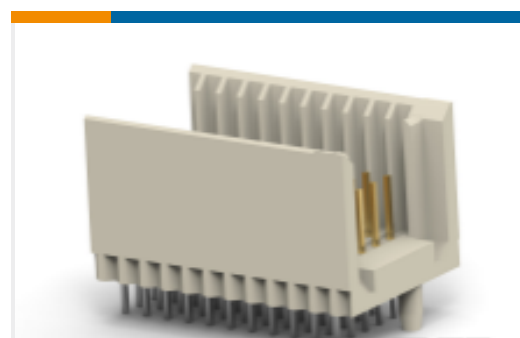
TE Part #5188399-1 Hard Metric Male Connector: Traditional Backplane, Mezzanine, 2mm
