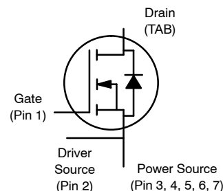
N-CHANNEL MOSFET
