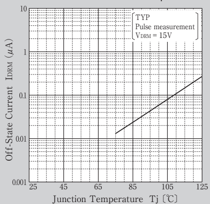
I_{DRM} - T_j 特性 Off-State Current vs Junction Temperature
