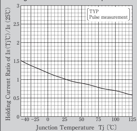
I_H - T_j 特性 Holding Current vs Junction Temperature
