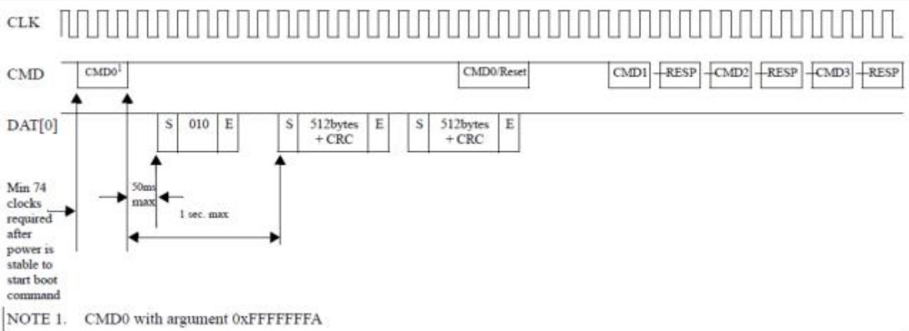
Boot operation complete Clock = 400 kHz (Compatible with the description which ≤400kHz)
