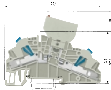
WKC 2.5 TKG/35 with fuse holder
