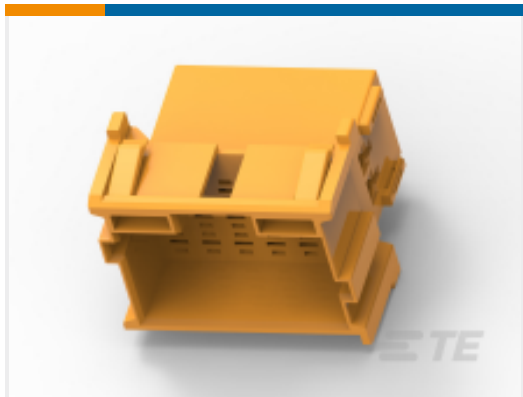
TE Part #6-967629-1 TAB HOUSING, 2.8MM, 18POS.
