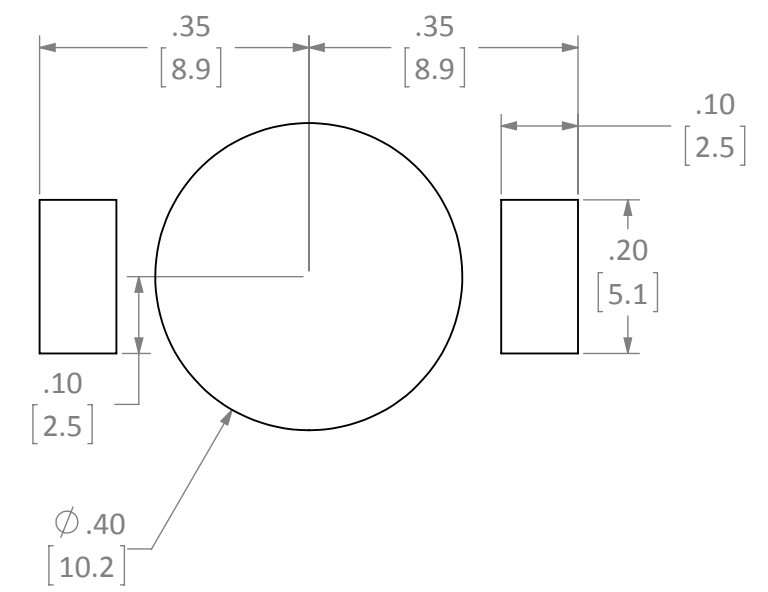
RECOMMENDED FOOTPRINT
