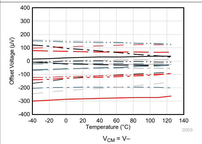
Figure 5-4. Offset Voltage vs Temperature
