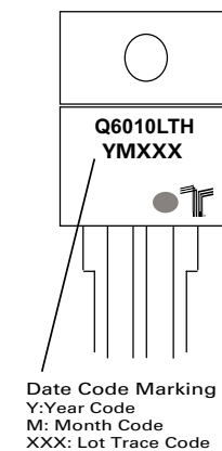
TO-220 AB - (L Package)
