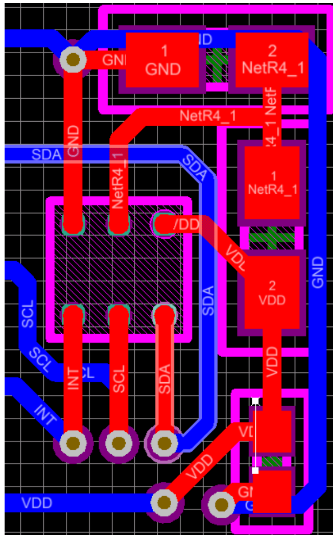
Figure 19. Layout
