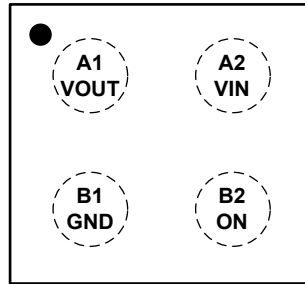
WLCSP-0.8×0.8-4B
